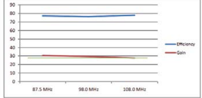
FMAMP650 Efficiency and Gain Idq=0,5A Vdc= 46
